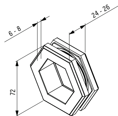
Hexagonal handle 8/84 3SRLM
