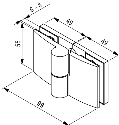
Folding hinge 8/65 13RLM
