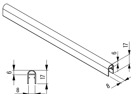
Seal (between the panels) 8/42 HXRLO
