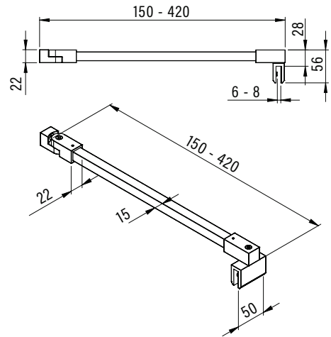
Standard shower rod 8/65 31RLM
