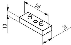
Extension plate 8/65 26RLM
