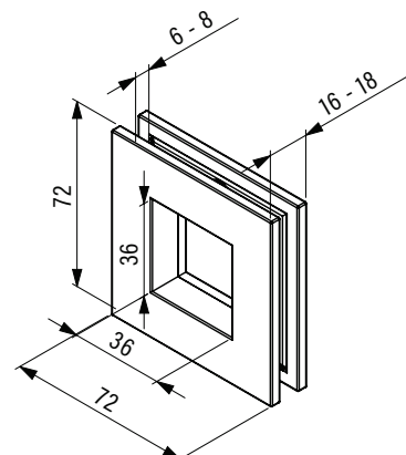
Square handle 8/84 0RRLM
