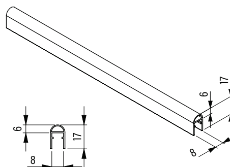
Seal (between the panels) 8/42 HXRLO
