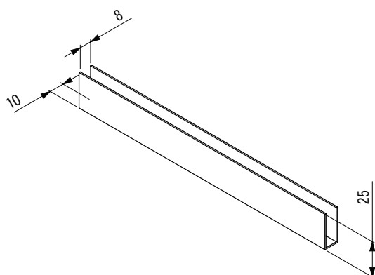
Steel profile 8/12 50RLM
