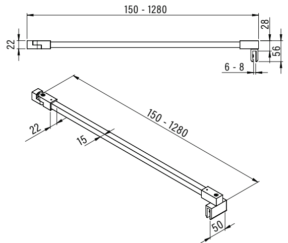
Long shower rod 8/65 32RLM
