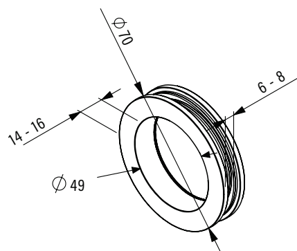
Round handle 8/84 0ORLM
