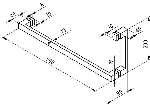
Towel handle 8/65 54RLM
