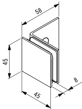
Wall mounted glass clamp 8/65 21RLM
