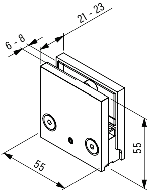
Floor mounted glass clamp 8/65 24RLM
