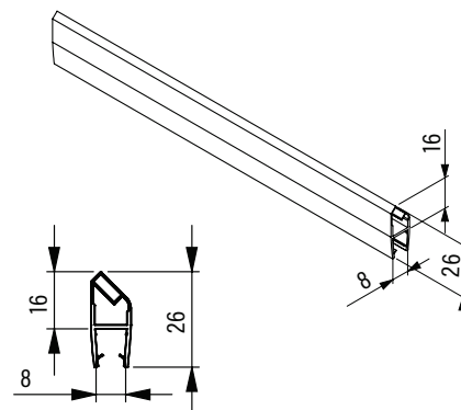
Magnet seal 8/42 8X2L0
