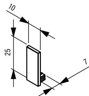
Profile end cap 4/83 99RLM
