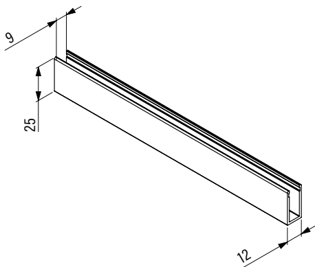
Aluminium profile 8/12 40RLM
